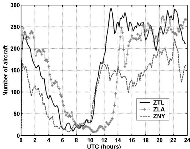
Fig. 4 Traffic count on 6 May 2003 in selected centers in the United States across a 24-hour period.
