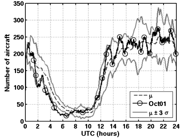
Fig. 11 Model-based average traffic counts and uncertainty bounds in the Fort Worth Center.
