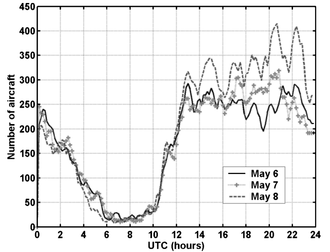
Fig. 5 Atlanta center traffic across multiple days.
