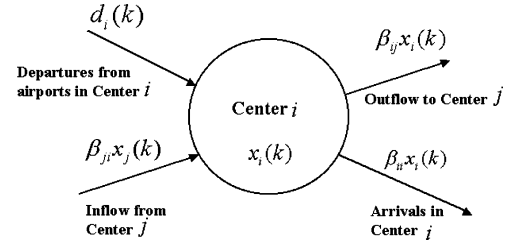
Fig. 3 Components of aircraft flow contributing to the traffic count in a given center.
