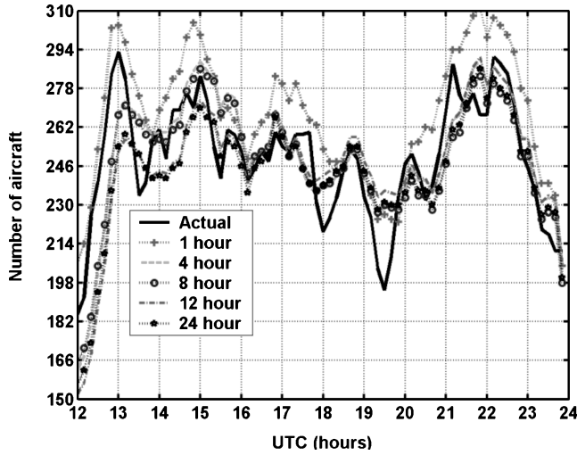
Fig. 6 Predicted aircraft counts in ZTL with u updated at every time step, but A aggregated over one-hour through 24-hour time intervals using 6 May 2003 data.
